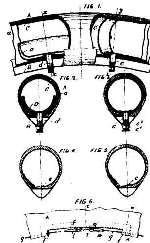
Seddon's Pneumatic Tire.
