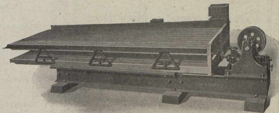
No. 9 Double-Deck Wilfley—Two Tables in the Floor Space for One
