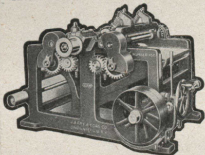
Our No. 156 Cabinet Planer.
