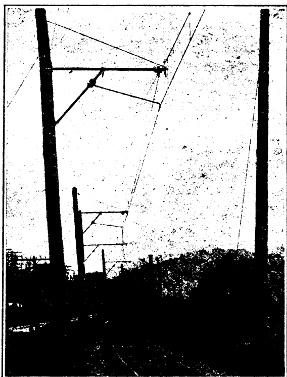
The Catenary Line Construction
