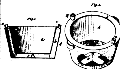
7797 Martin &amp; Burgert's Improvements in Dough Troughs.
