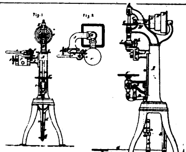
7798 Walsh &amp; Bowen's Metal Can Seaming Machine.
