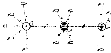
13006 Watson's Improvements on Telephone Circuits.
