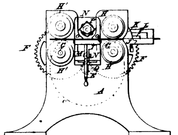
13008 Naylor's Improvements on Machines for Dressing Barrel Hoops, &amp;c.
