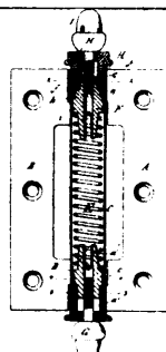
13001 Warden's Improvements on Butt Hinges.
