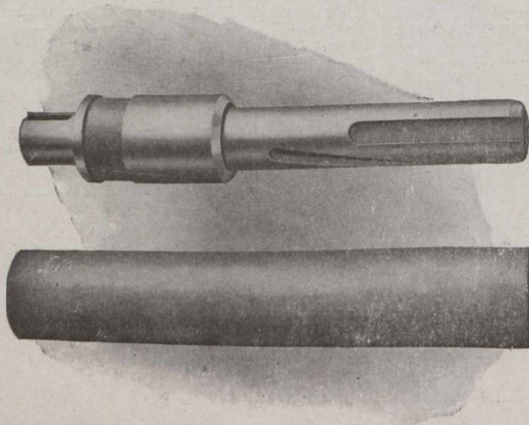
Above, finished "DR6" Piston; below, solid alloy steel bar from which the piston is turned, milled and ground.
