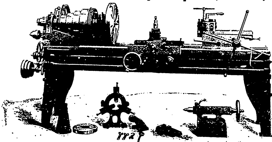
Engine Lathe with Turret Attachment.
