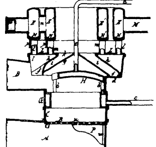
2324 Gommenginger's Improvements on Hot Air Furnaces.
