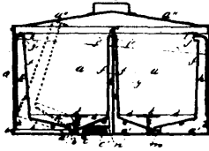
2320 Davis's Washing Machine.
