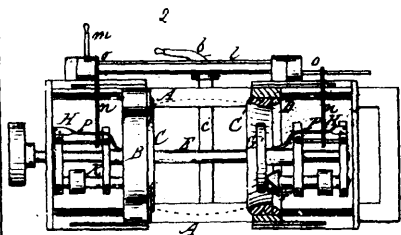
2325 Greenwood's Machine for Crasing and Chamfering Barrels.
