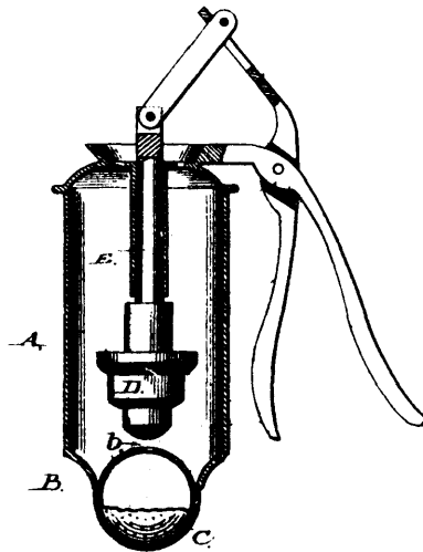
21171 Goldman's Sprinkler and Atomizer.
