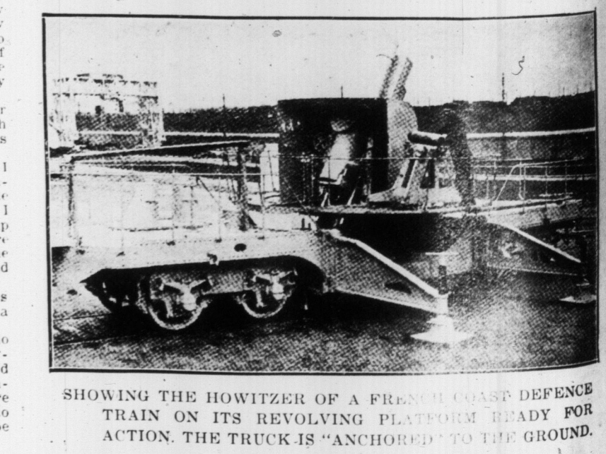
SHOWING THE HOWITZER OF A FRENCH COAST DEFENCE TRAIN ON ITS REVOLVING PLATFORM READY FOR ACTION. THE TRUCK IS "ANCHORED" TO THE GROUND.
