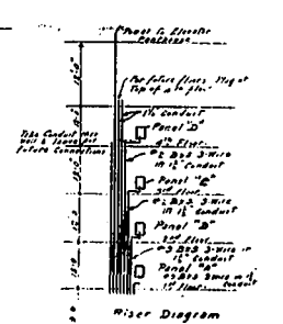
Riser Diagram
