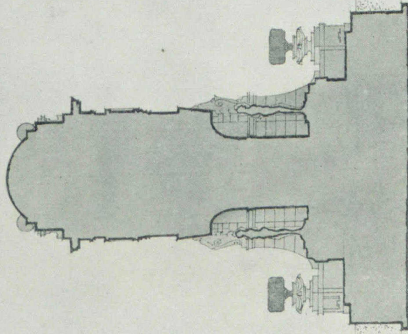
♦ SECTION ♦
