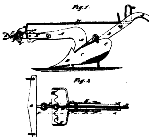
5723 Miller's Improvements on Plough-clevises.
