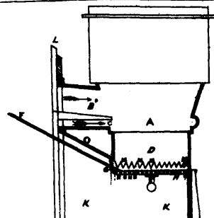
5730 Laidlaw's Hot Air Furnace.
