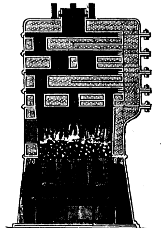
Sectional View.
