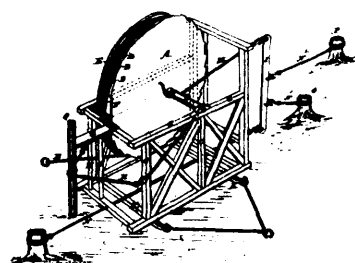
12255 Norcott's Improvements on Stump Extractors.
