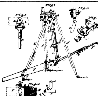
12257 Augspurger's Improvements on Drag Sawing Machines.
