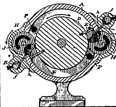
22934 Sewrey's Rotary Engine.
