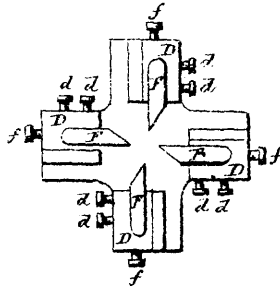
3007 Hine &amp; Dibble's Machine for Threading Bolts.
