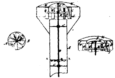
3008 Conklin's Improvements on Engine Smoke Stacks.
