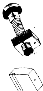
13455 Martel's Improvements on Nut Locks.
