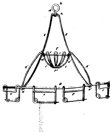
34959 Smith's Combined Bag, Twine and Sample Holder.
