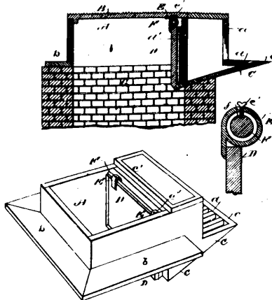
34955 Smith's Combined Culvert Top and Trap.
