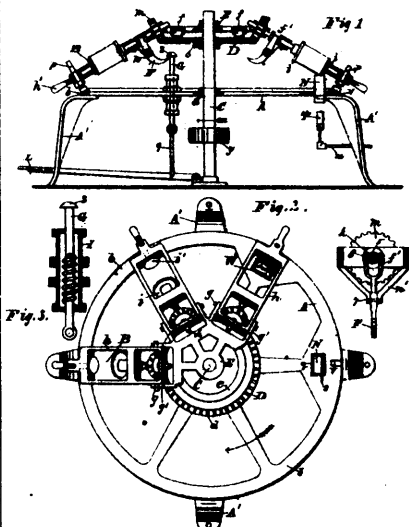
Jones and Thurber's Can Soldering Machine.
