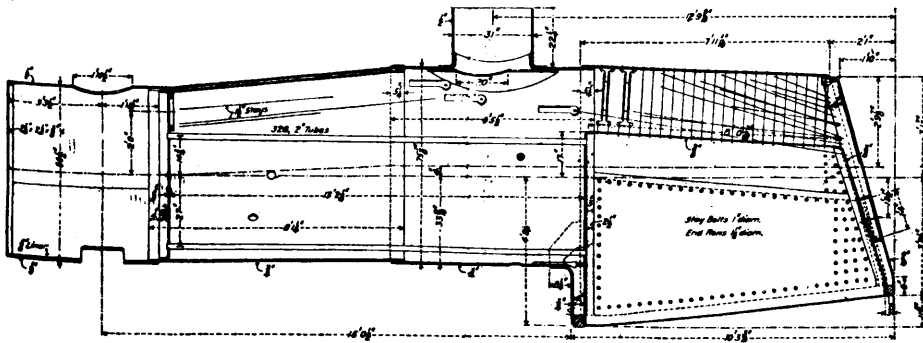
BOILER OF C. P. R. TWO-CYLINDER COMPOUND.
