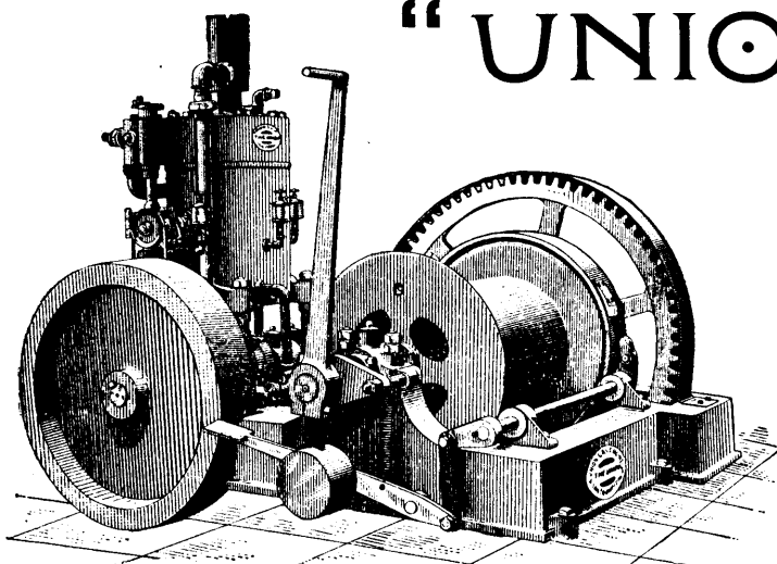
UNION GAS OR OIL ENGINE & HOIST COMBINED—On Strong Iron Base. 6 to 50 h.p. of design shown in cut.
