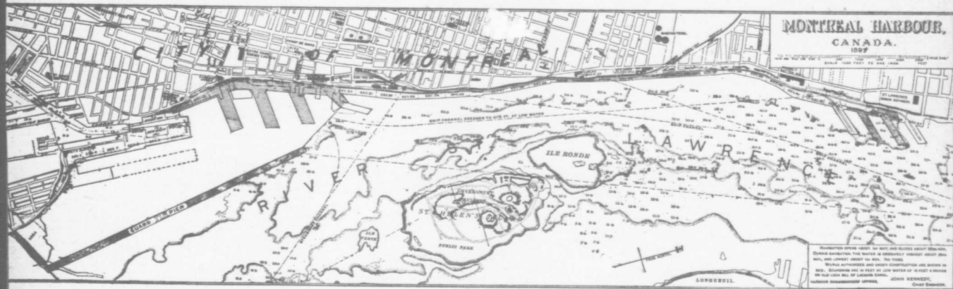
GENERAL PLAN OF MONTREAL HARBOUR SHOWING PROPOSED IMPROVEMENTS.
