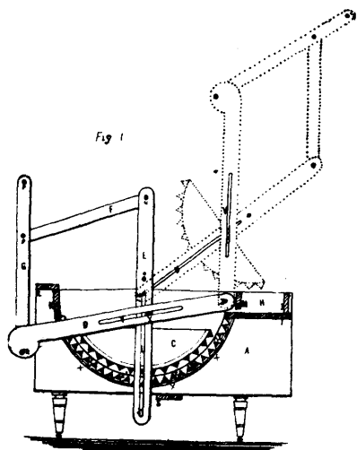
33804 Patchel's Pump.
