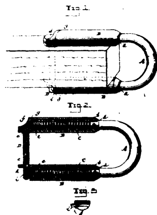
27064 Morey's Clevis for Attaching to Plough Beams, etc.
