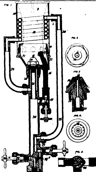
27059 Hattway's Spray Lamp or Burner.
