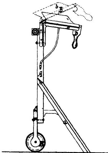
27063 Hogarth's Bag Holder and Truck.
