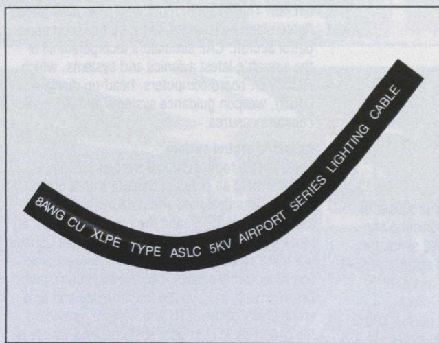
Series cable for airport runway lighting system
