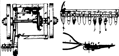
4811 Atwood's Mowing Machine.
