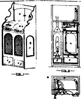
4814 Maltus' Street Car Fare Box.
