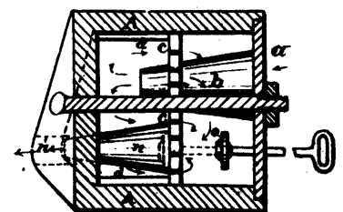
4816 Taylor & Sutherland's Blacksmith's Tuyere.
