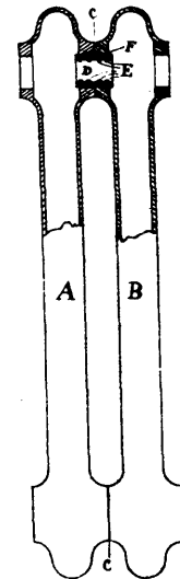
32629 King's Steam or Hot Water Radiator.
