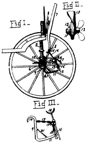
32624 Mayne's Carriage Tongue Support.
