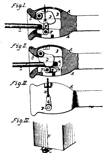
32632 Everitt's Car Coupling.
