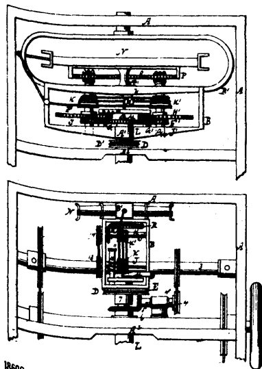
18692 Brownell's Machine for making Twin Cordage, &c.
