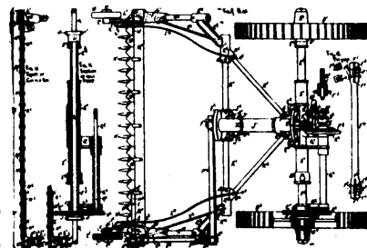
14222 Levalley's Improvements in Mowing Machines.
