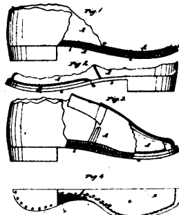
14211 Lewis's Improvement in Boots and Shoes.
