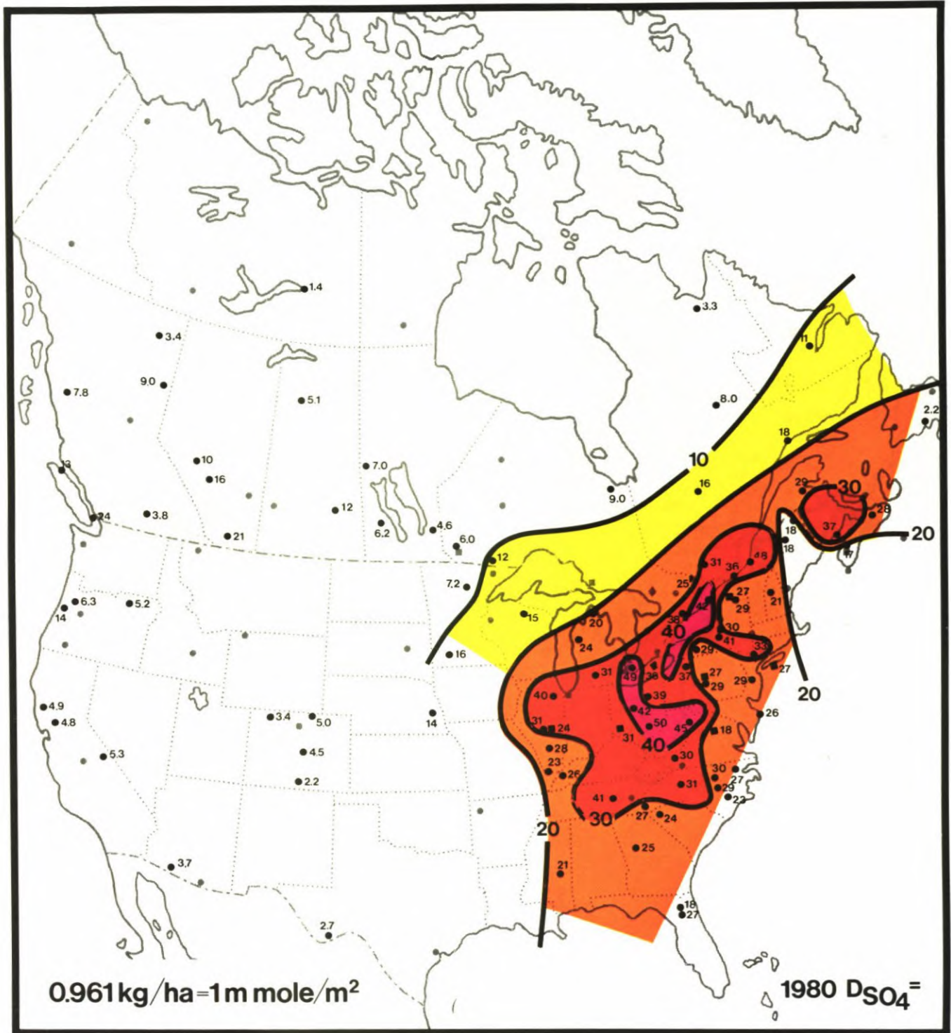
Precipitation amount- weighted mean sulfate ion deposition for 1980 (m moles per square meter)
