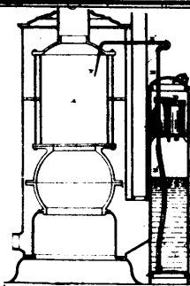
9246 Quackenboss' Railway Car Stove Fire Extinguisher.
