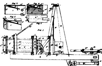
9252 Phillips & Jones' Improvements on Baling Presses
