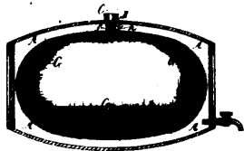
9244 Steen's Apparatus for Preventing Air Entering Casks.
