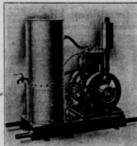
The Empire Engine No. 2, 2 Horse Power
