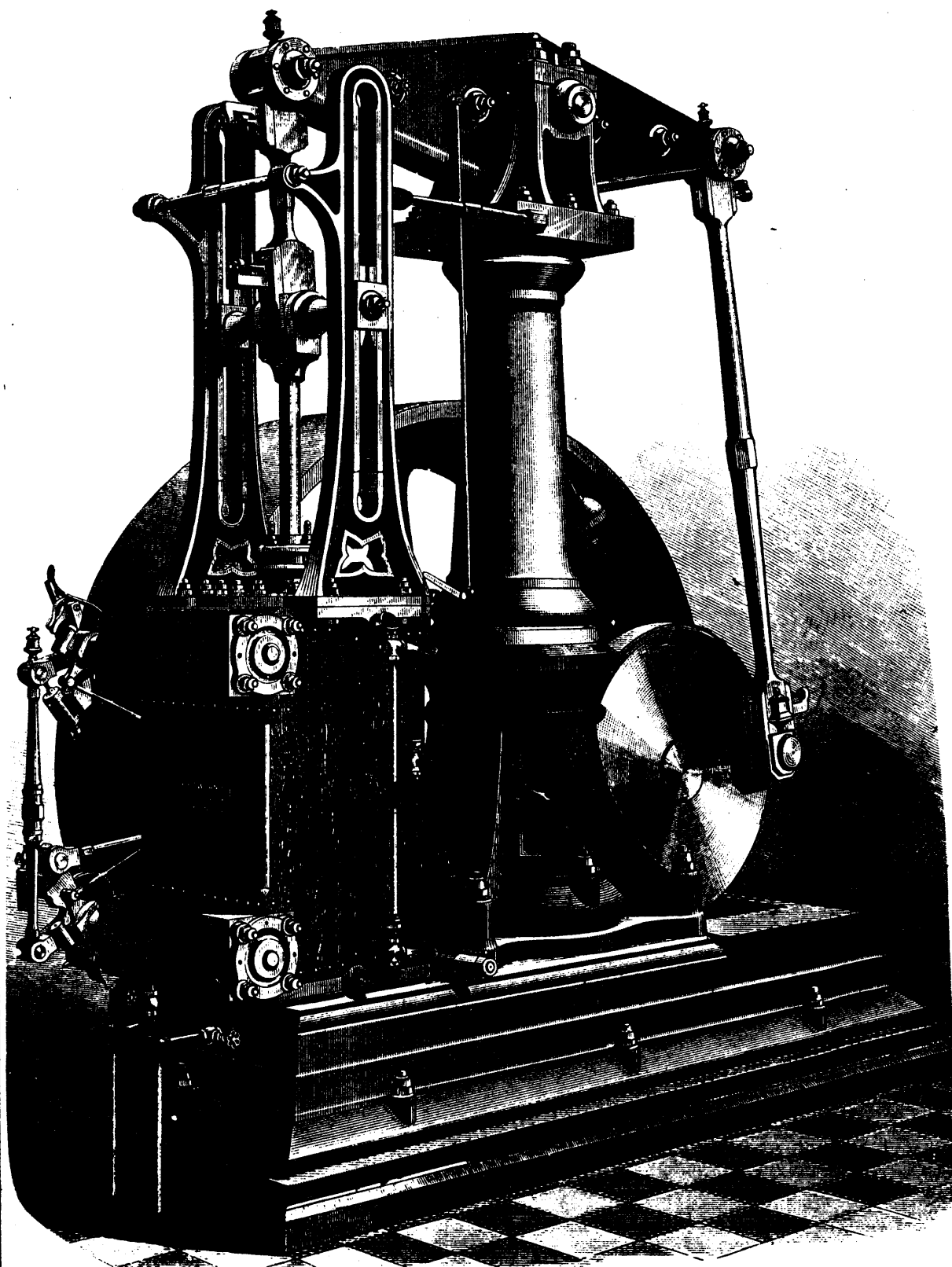
NEW BEAM ENGINE BUILT AT THE CONTINENTAL WORKS, GREENPOINT, BROOKLYN, N. Y.
