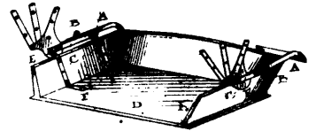
10150 Conboy's Adjustable Seat Rail for Carriage Tops.
