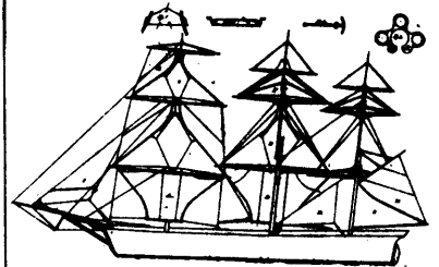
10153 Flowers' Improvements in Sails.
