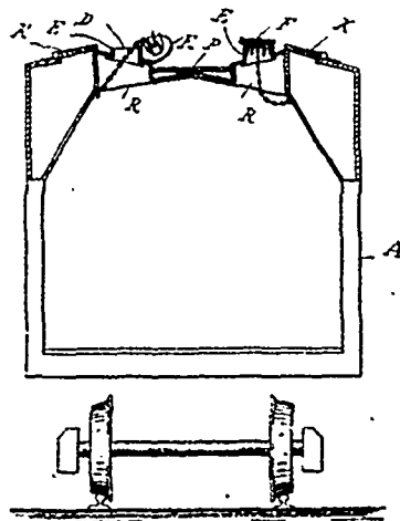
29300 Balnes' Stock Car.
