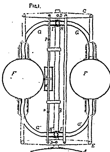
29298 Austin's Feeder for Steam Rollers.
