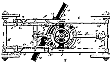
29291 Moate's Road Grader.
