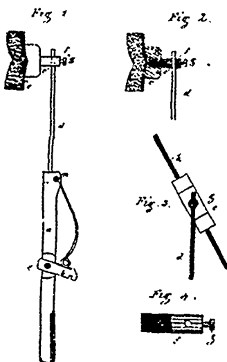
29302 Herberg's Damper for Upright Pianos
