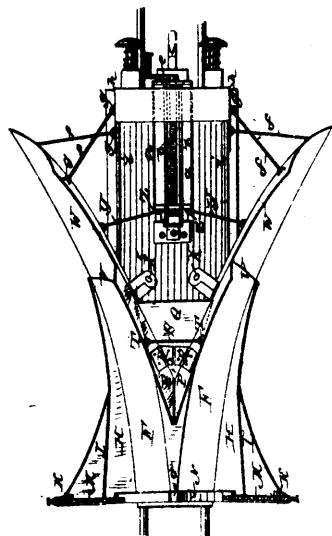
16059 Hesselbom's Improvements on Snow Ploughs.
