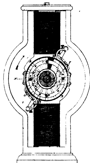
16056 Hochhansen's Improvements on Dynamo or Magneto Electric Machines.
