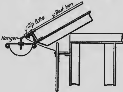
Hanging Gutters "D.B." Adjustable Strap Hanger.
