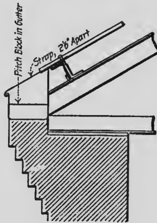
Details of Box Gutter.
