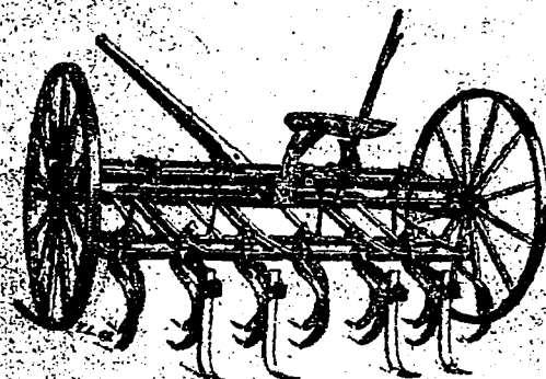
MASSEY-HARRIS CULTIVATOR.
