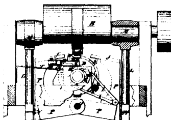
3121 Wilmot's Improvements on the Manufacture of Metal Tubing.
