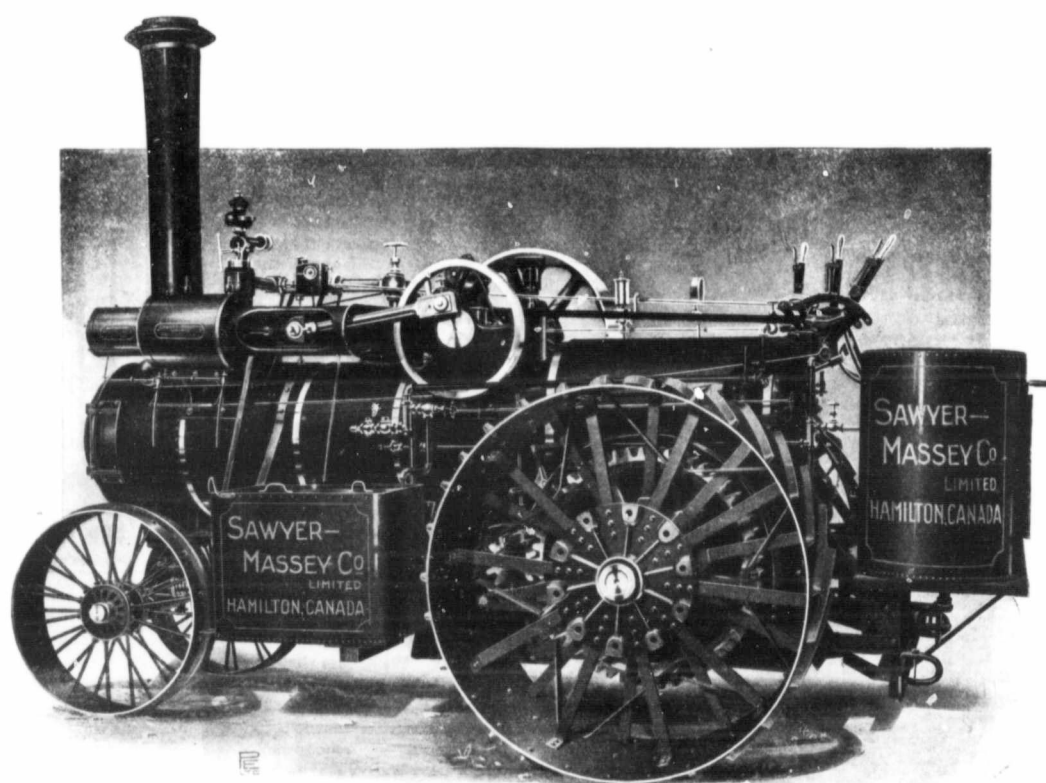
New Model S-M Combination Plowing and Threshing Engine, Manufactured in 27, 30 and 32 H. Powers.
