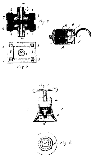
38754 McCarthy's Insulator.
