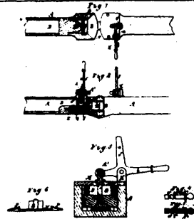
3522 Wiewell's Improvements on Car-Couplings.
