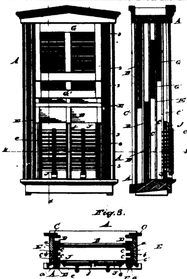
19191 Hill's Sliding Window Blind.
