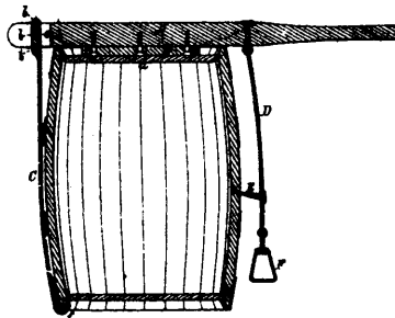
2424 Griffin &amp; Smith's Machine for Heading Barrels.
