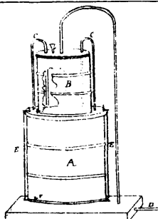
2426 Hicks &amp; Parish's Process and Machine for the Manufacture of Gas.
