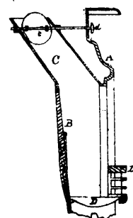
2435 McCallum &amp; Moffat's Portable Parlor Grate.
