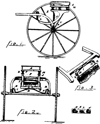
33522 Brownell's Road Vehicle.
