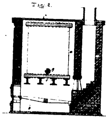
33521 Pitt's Apparatus for Distilling and Deodorizing Petroleum.
