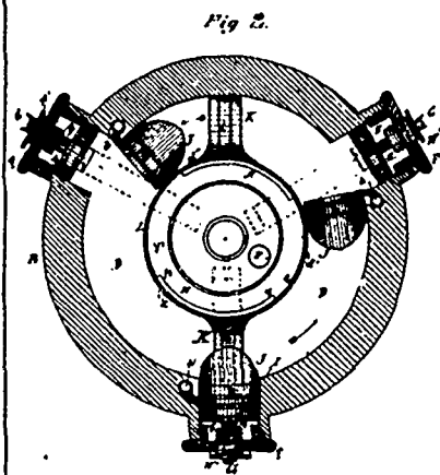
28368 Broughton's Rotary Engine.
