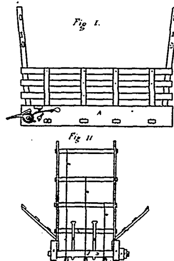
28374 Hughson's Binder for Vehicle Racks.
