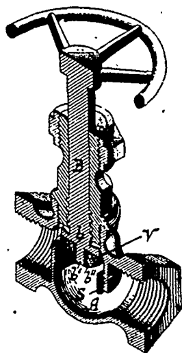
28369 Traylor's Valve, Valve Seat, etc.
