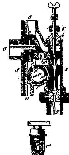
24363 Hogue's Injector for Steam Boilers.
