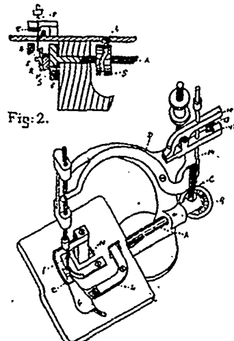
24360 Tucker's Sewing Machine.
