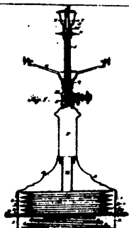
No. 1705. Mead's Hydro-carbon Vapor Lamp.
