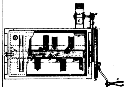
No. 1704. Holmes' Churn.
